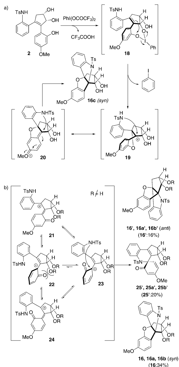
Scheme 3. Working model for the diastereoselectivity observed in the hypervalent iodine mediated oxidative double cyclization.
