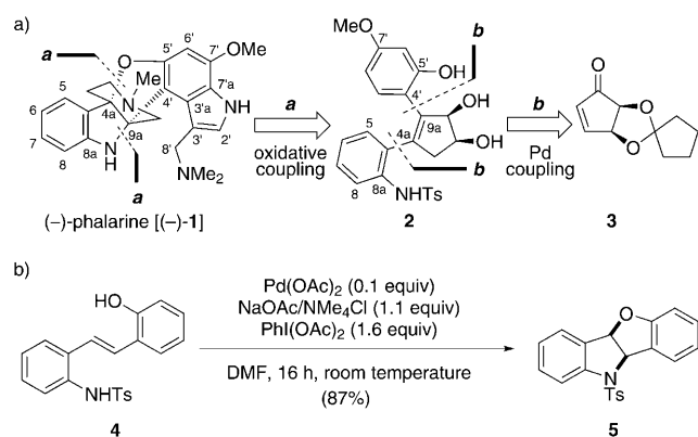
Scheme 1. a) Molecular structure of (–)-phalarine [(–)-1] and retrosynthetic analysis leading to 2 and 3 . b) Palladium-catalyzed tandem C–N and C–O bond formation reported by Muniz [4a] leading to 5 . DMF = N,N -dimethylformamide, Ts = toluenesulfonyl.
